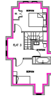
PROPOSED SECOND FLOOR (1:50)
