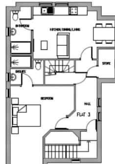
EXISTING FIRST FLOOR (1:50)
