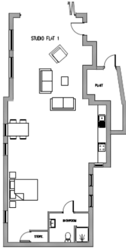
EXISTING BASEMENT (1:50)
