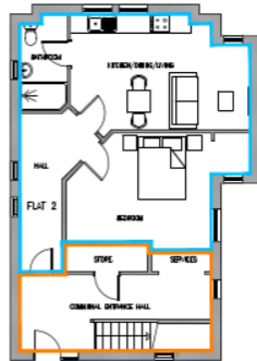
PROPOSED GROUND FLOOR (1:50)
