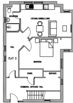
EXISTING GROUND FLOOR (1:50)
