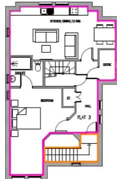
PROPOSED FIRST FLOOR (1:50)
